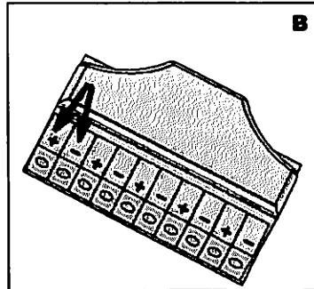
Figure B- Pay special attention to the polarity of each terminal, they alternate ground and positive.
